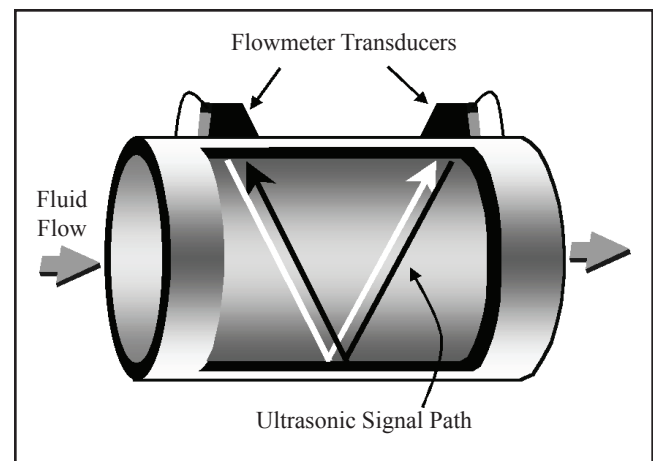
Figure 2. Transit-time ultrasonic flow meter measurement technique.
