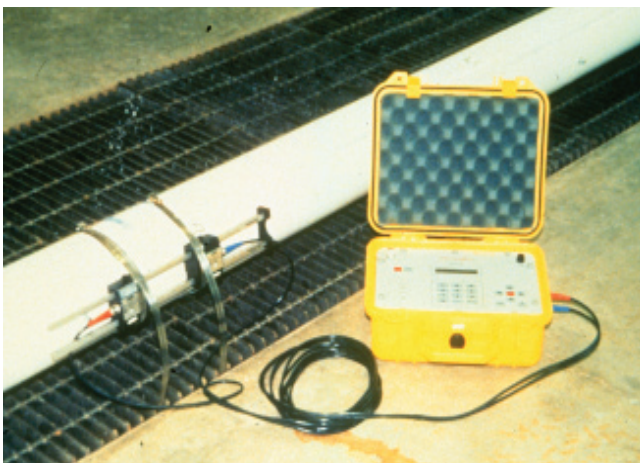
Figure 1. Transit-time ultrasonic flow meter.
