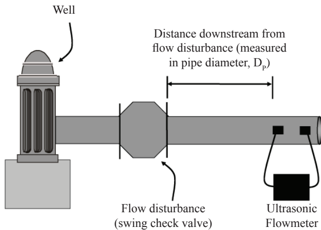
Figure 3. Schematic illustrating a typical irrigation system piping configuration.
