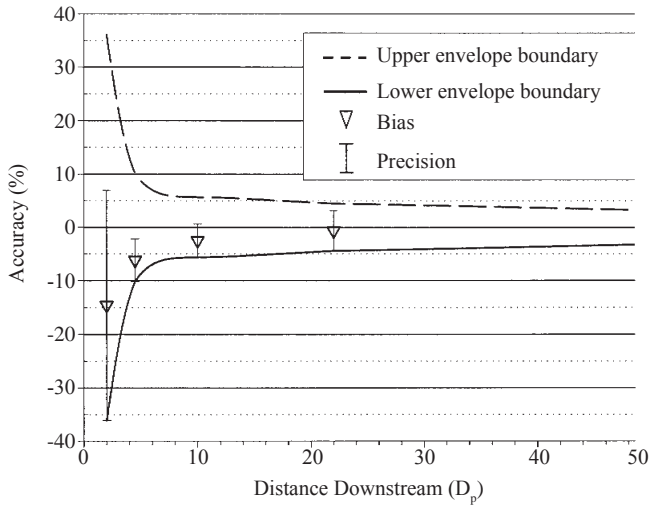
Figure 4. Ultrasonic flow meter performance envelope.
