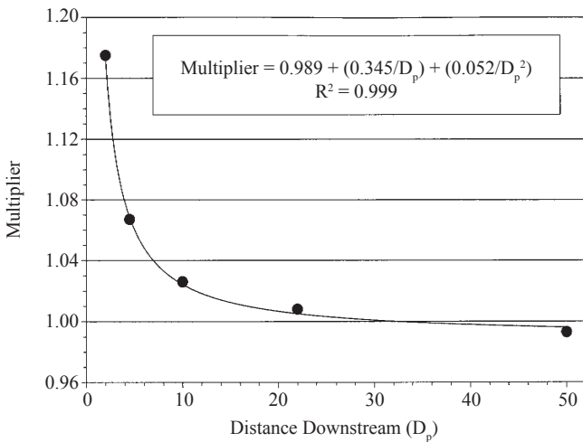
Figure 5. Bias-correcting multiplier.
