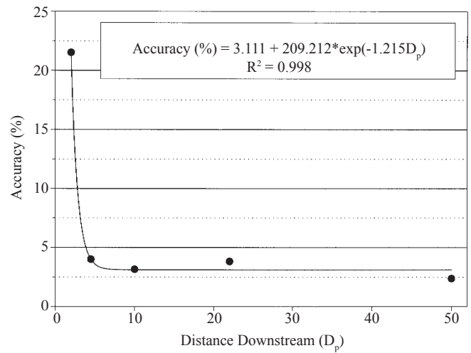
Figure 6. USFM accuracy with bias removed.
