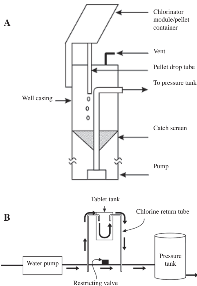
Figure 3. Tablet type chlorinators.
